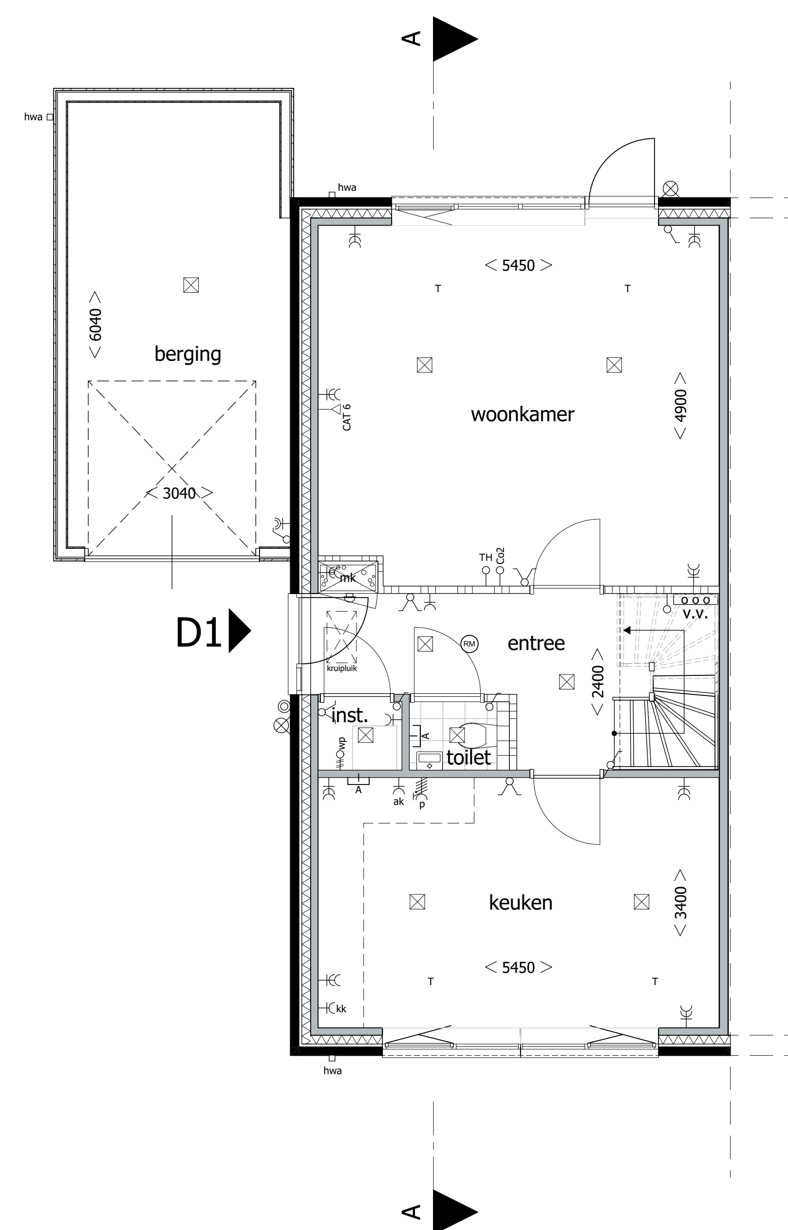
Begane grond type D1
