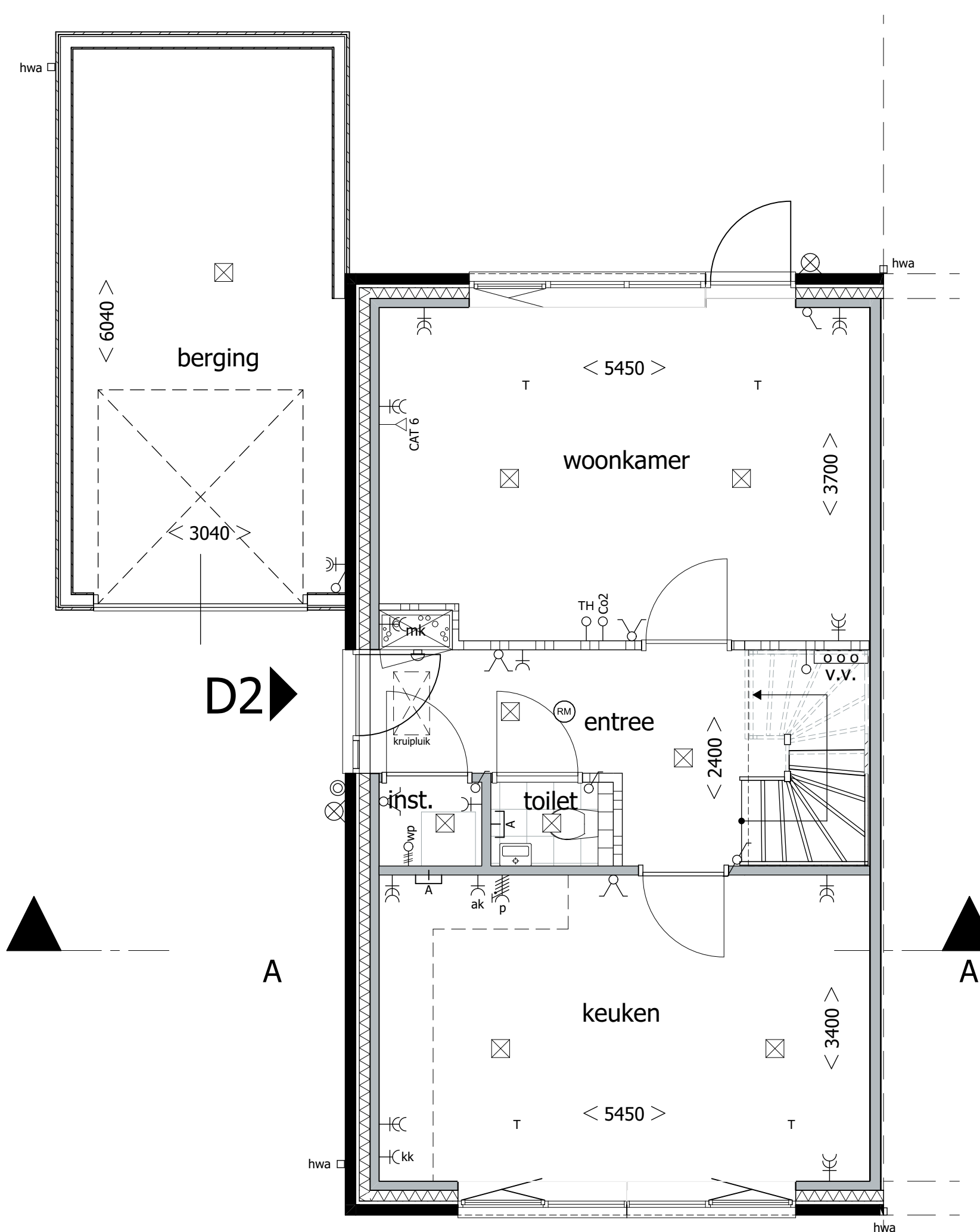
Begane grond type D2
